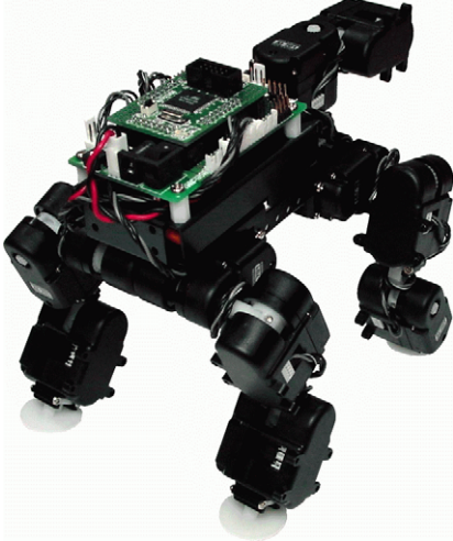
Figure 17. 4-legged robot
